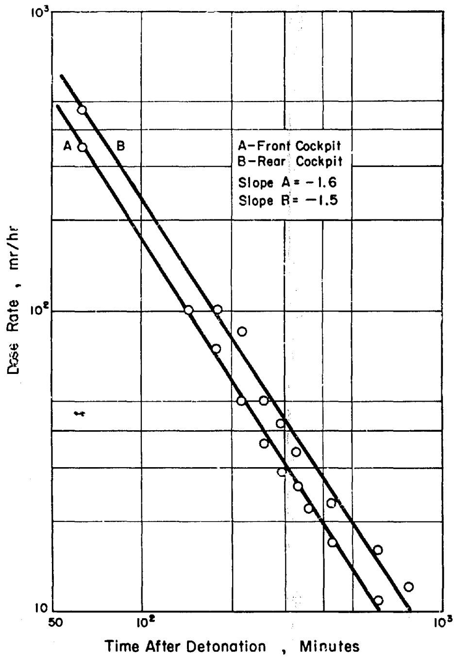
Figure 3.6 Decay of radiation dose rate in cockpit of contaminated aircraft, Shot Zuni, aircraft no. 527.
